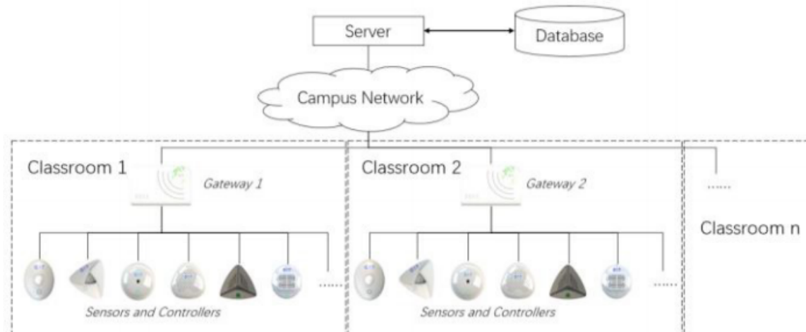
Figure. 1. Architecture Diagram
